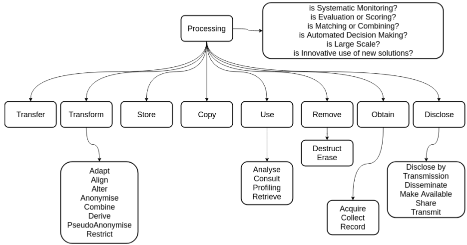
Fig. 4. Categories of Data Processing in DPV
