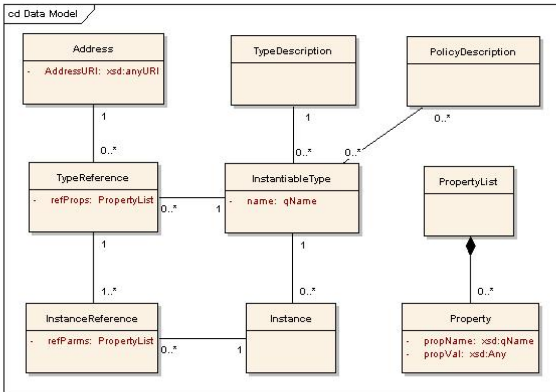
Figure 1 - Endpoint Reference Data Model
